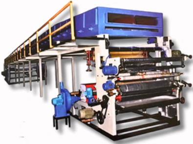
BOPP SELF ADHESIVE TAPE COATING & LAMINATION PLANT
