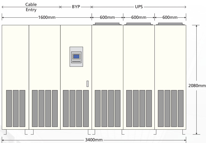
Capacity 1.05 MW UPS Footprint
