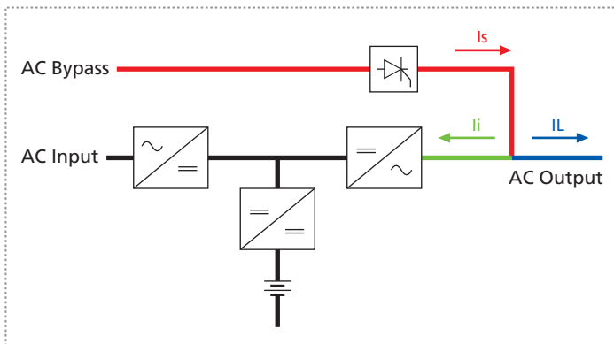
Smart Drive Mode of Operation
