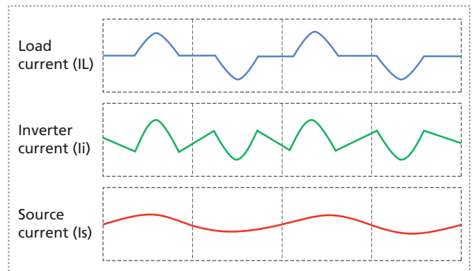
Smart Drive Active Power Compensation
